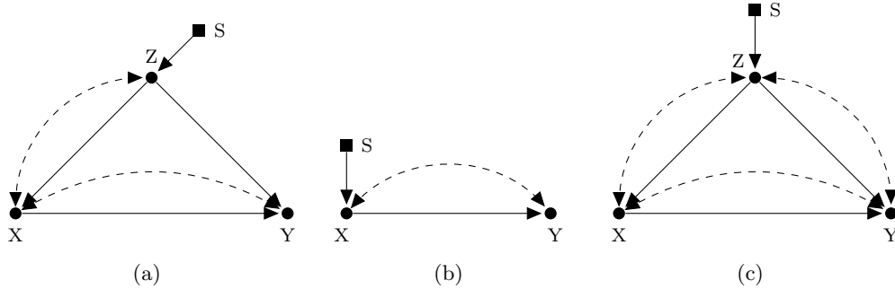
Figure 9: Examples of selection diagrams for the transportability task.
