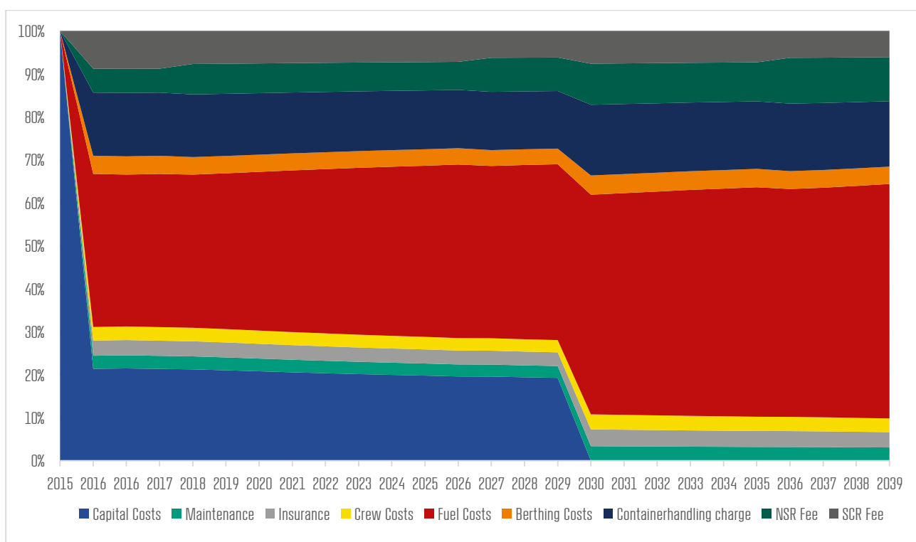
Figure 5.9: Total cost component breakdown for the 8000 TEU ice reinforced vessel
