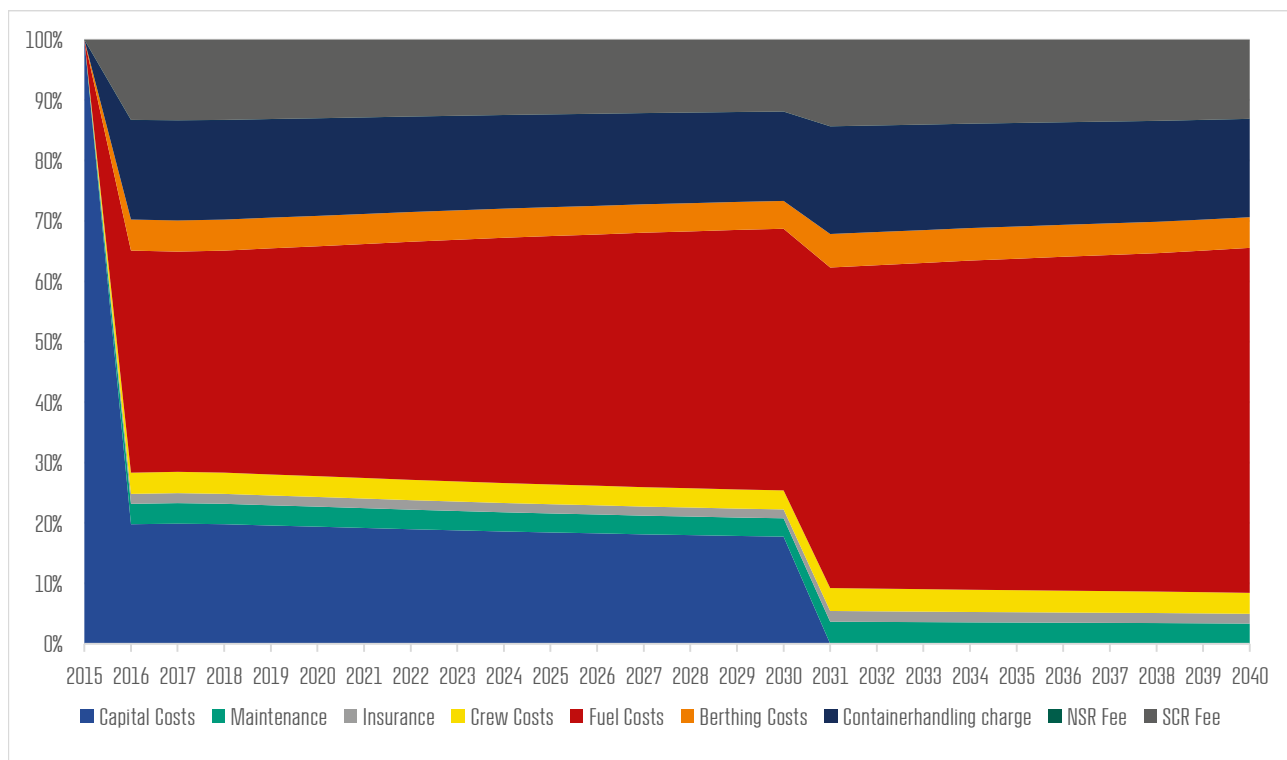
Figure 5.8: Total cost component breakdown for the 8000 TEU open water vessel
