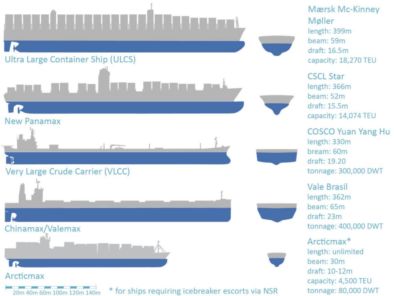
Figure 5.3: Size comparison of Arcticmax and large open water vessels Source: The Arctic Institute
