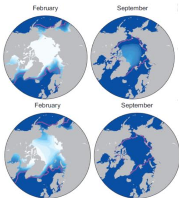
Figure 3.3: Projected Arctic sea ice concentration in 2080-2100
