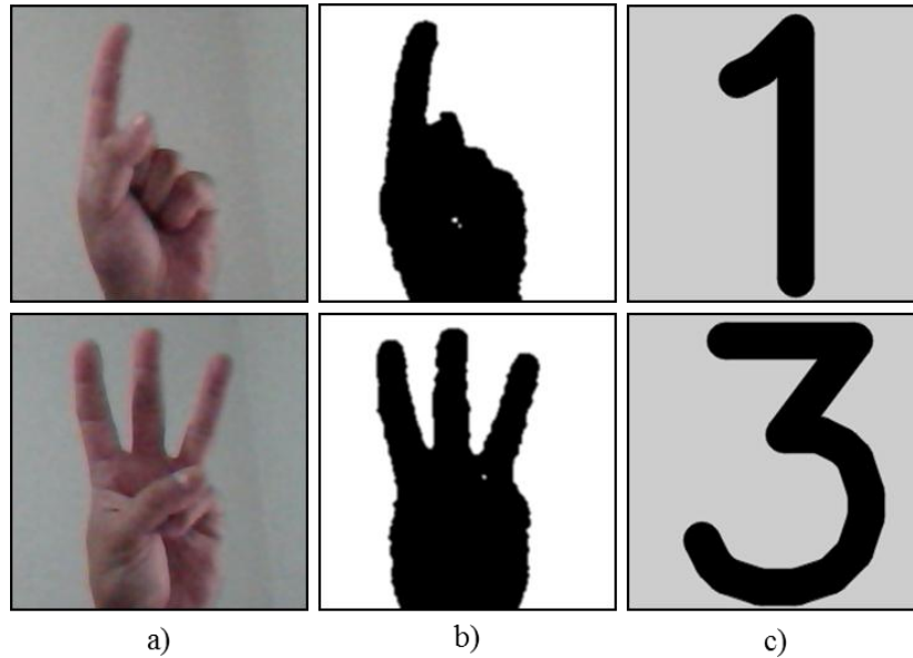
Fig. 10. a) Captured frame b) segmented image c) classification result
