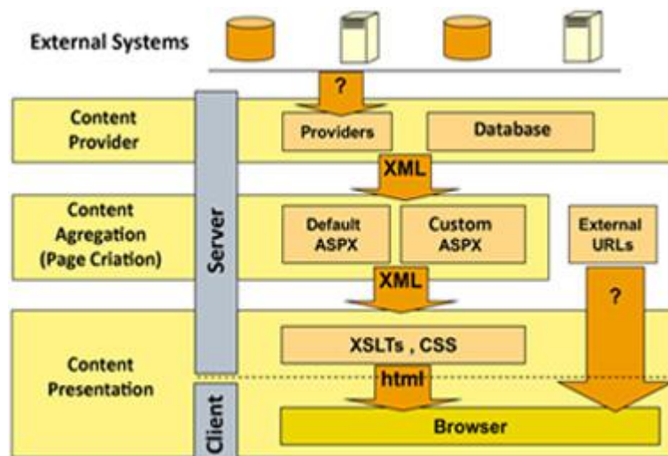
Fig. 2. Framework WIZY Layers
