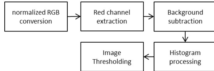
Fig. 3. Key steps of segmentation
