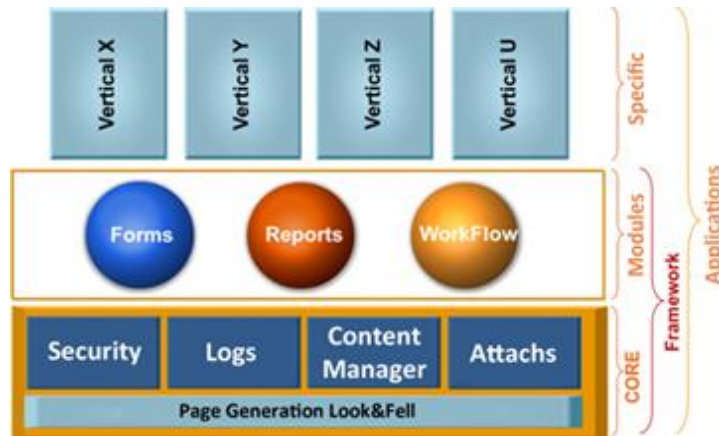
Fig. 1.Wizy Structure Organization
