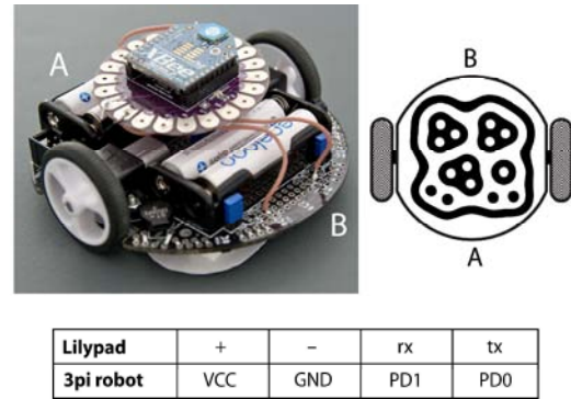
Figure 3. A Pololu 3pi robot with a XBee module mounted in a Lilypad XBee. The table shows how the module is connected to the robot. A and B indicate how the fiducial should be oriented on the bottom of the robot.
