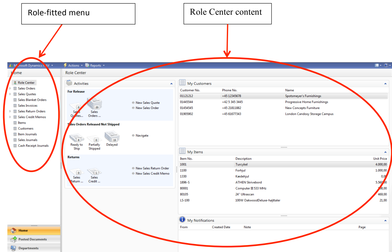
Figure 4. User interface of NAV 2009 RTC. Copyright of Microsoft Corp.
