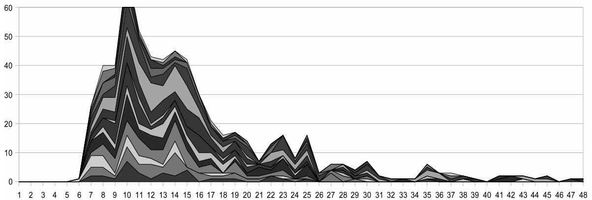
Figure 4. Distribution of object-size/fixation length \{length(F_j), size(O_j)\} . The X-axis shows the number of samples per fixation; the Y-axis the number of fixations counted in the data set; each color in the graph represents a different object size. Most fixations contain between 9 and 16 samples; with a sampling rate of 50 Hz, this equals fixation length of 180 to 320 ms.
