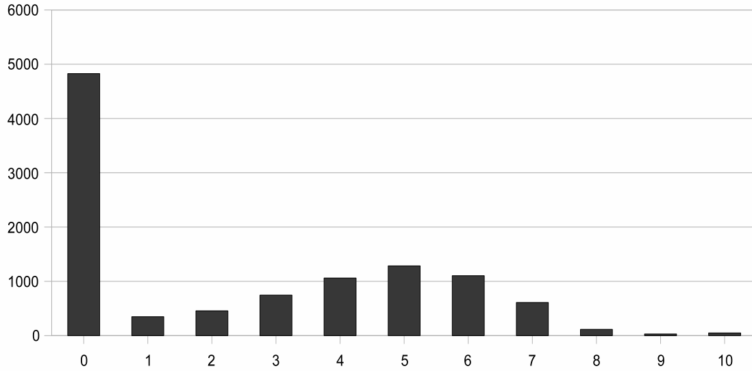
Figure 1. Distribution of sample-object distances dist(O_j, S_i) in the data according to equation (3). Note that distances on the X-axis are on a logarithmic scale. The classes 1 to 7 represent sample-object distances of up to 1, 2, 4, 7, 12, 19 and 32 pixels respectively. Most samples are in the textual objects' box (class 0) while there is a peak around \sqrt{e^4} to \sqrt{e^5} = 7 to 12 pixels distance between the sample points and the object's outer border.
