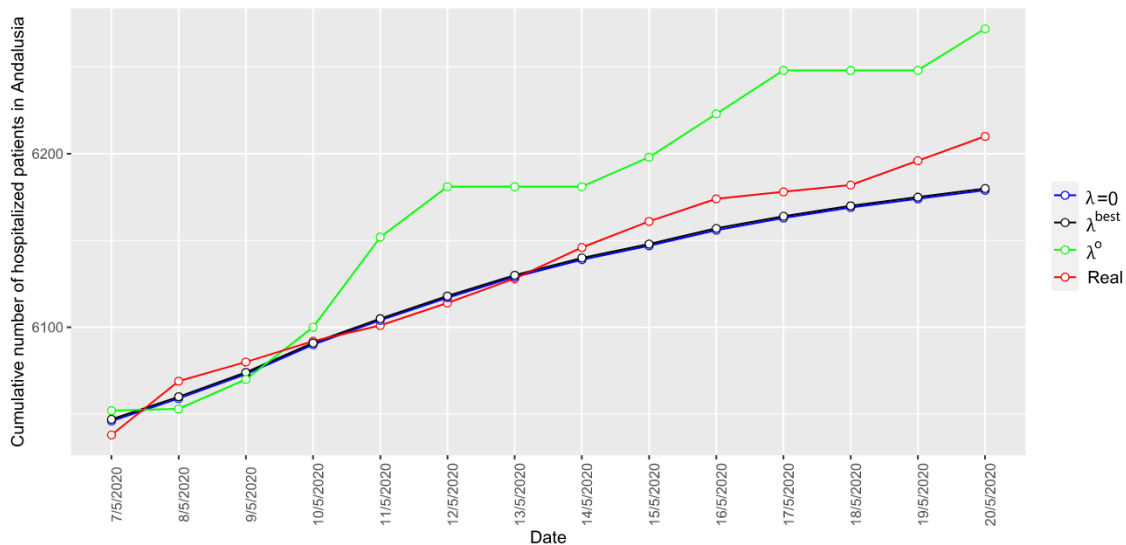
Fig. 10. Fourteen-day-ahead predictions for the cumulative number of hospitalized patients in Andalusia for COVID-19 in Testing Period 3 for three values of the tradeoff parameter \lambda , together with the actual values of the variable. (For interpretation of the references to color in this figure legend, the reader is referred to the web version of this article.)
