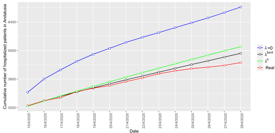
Fig. 9. Fourteen-day-ahead predictions for the cumulative number of hospitalized patients in Andalusia for COVID-19 in Testing Period 2 for three values of the tradeoff parameter \lambda , together with the actual values of the variable. (For interpretation of the references to color in this figure legend, the reader is referred to the web version of this article.)
