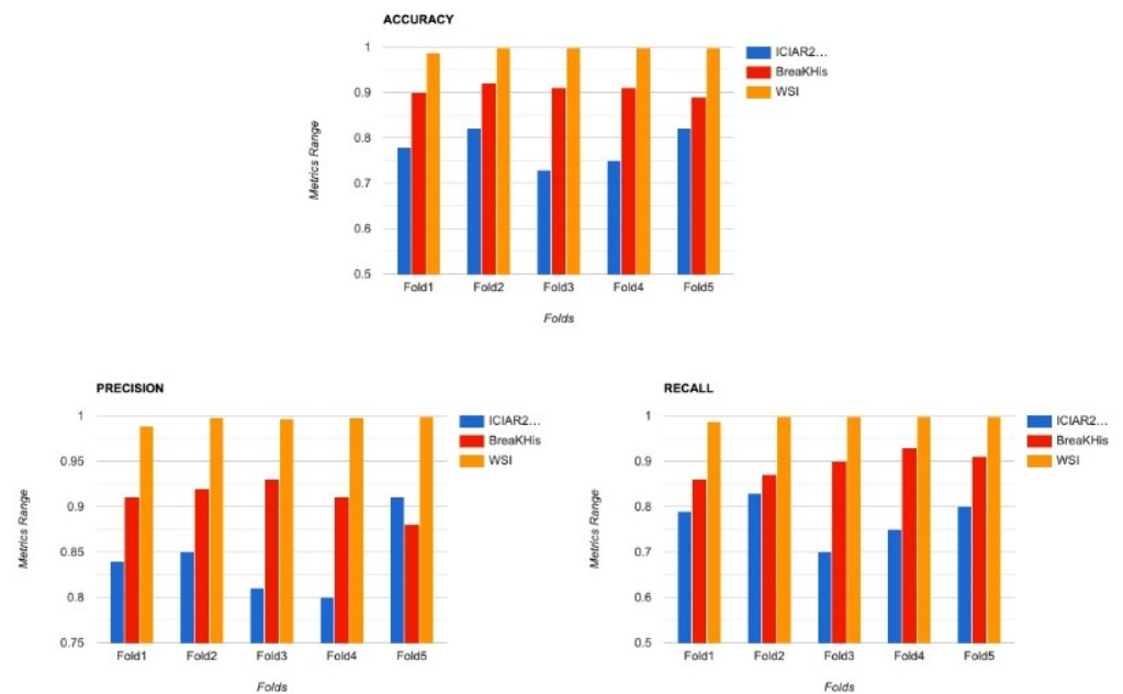
Figure 6. Comparison of performance metrics for WSI(O), BreakeHis(R), and ICIAR2018(B) Datasets.
