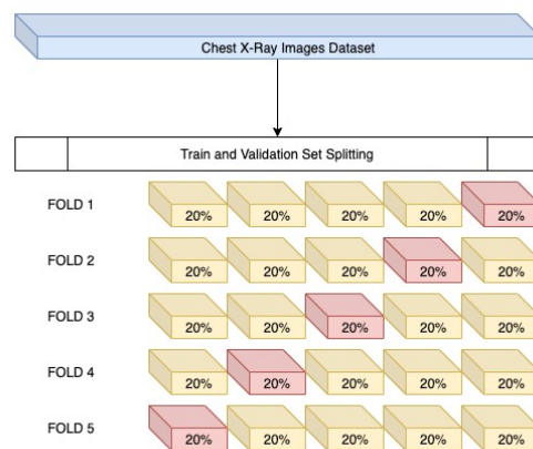
Figure 14. Cross validation.
