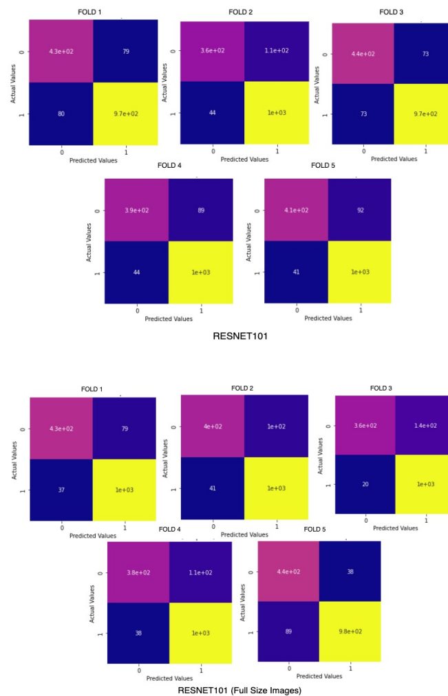
Figure 3. ResNet101 on BreCaKHis on cropped ( above ) and original sized images ( below ).
