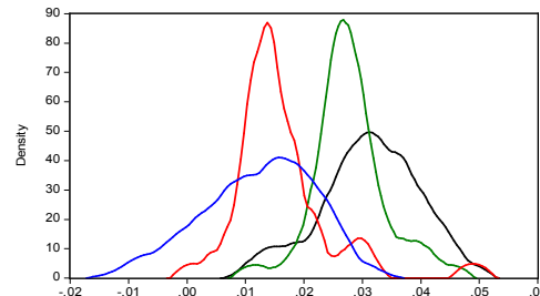
Figure 3. Kernel Distribution
