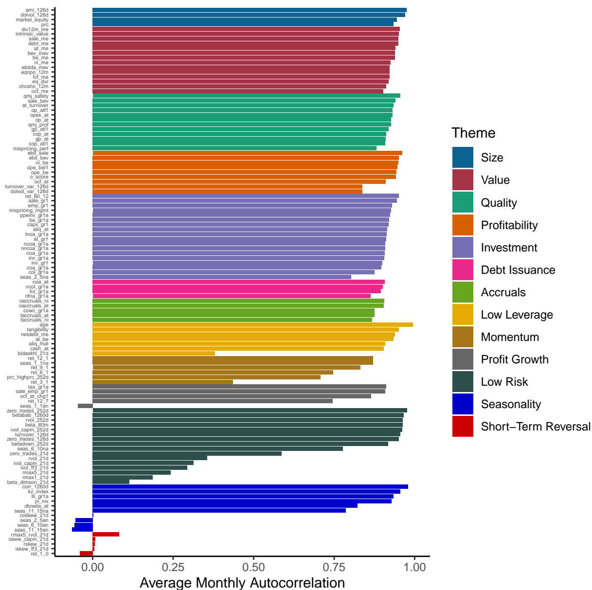
Figure C.2: Feature Autocorrelation
