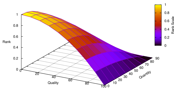
(b) Rank method setting \alpha and \beta to two
