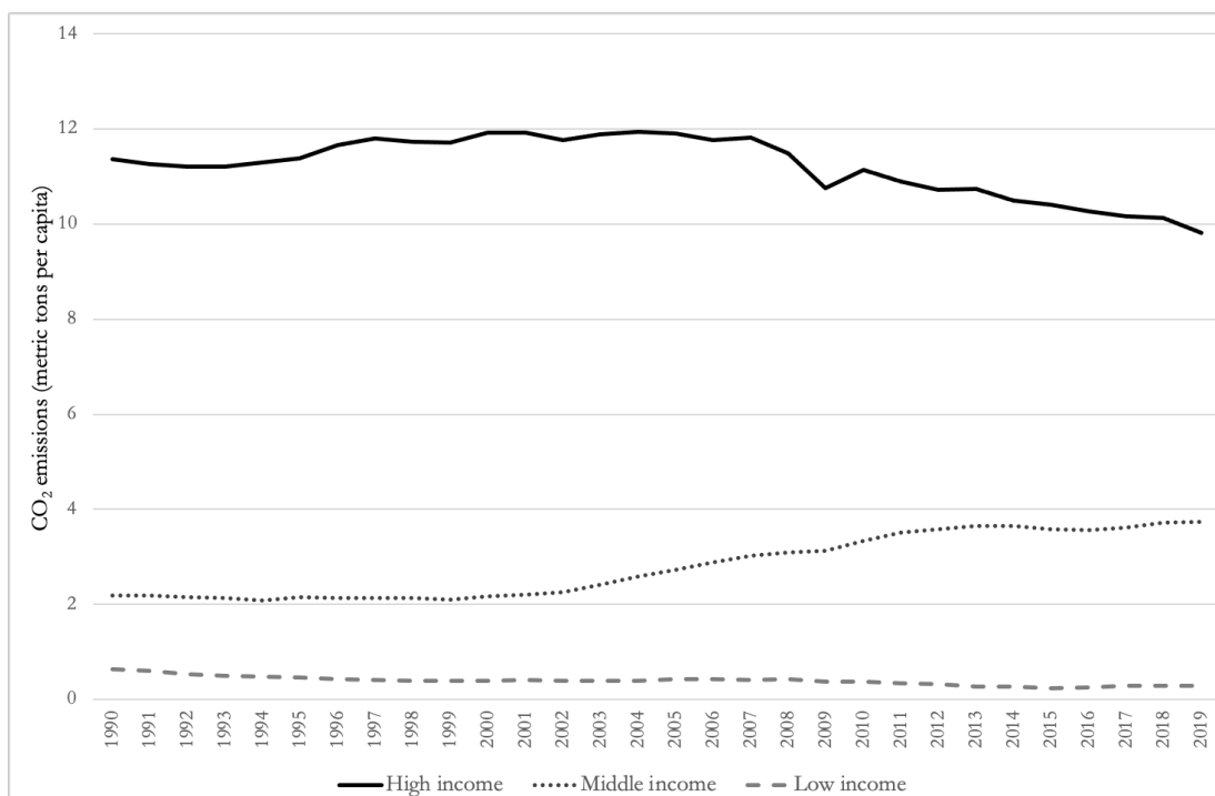
Figure 1a: CO2 emissions (mt) per capita
