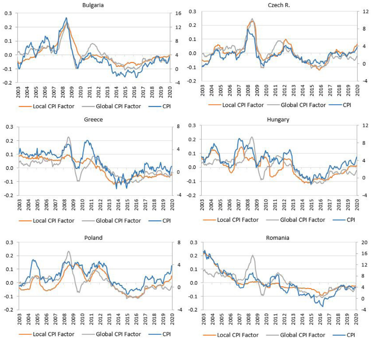
Fig. 2. Co-movement of actual inflation rates with local and global CPI factor estimated using the PLS approach. Notes: This figure plots the actual inflation rates along with local and global inflation factors where the factors are calculated as the first common component of the PLS approach utilizing the disaggregated CPI and all country-level headline inflation rate data.
