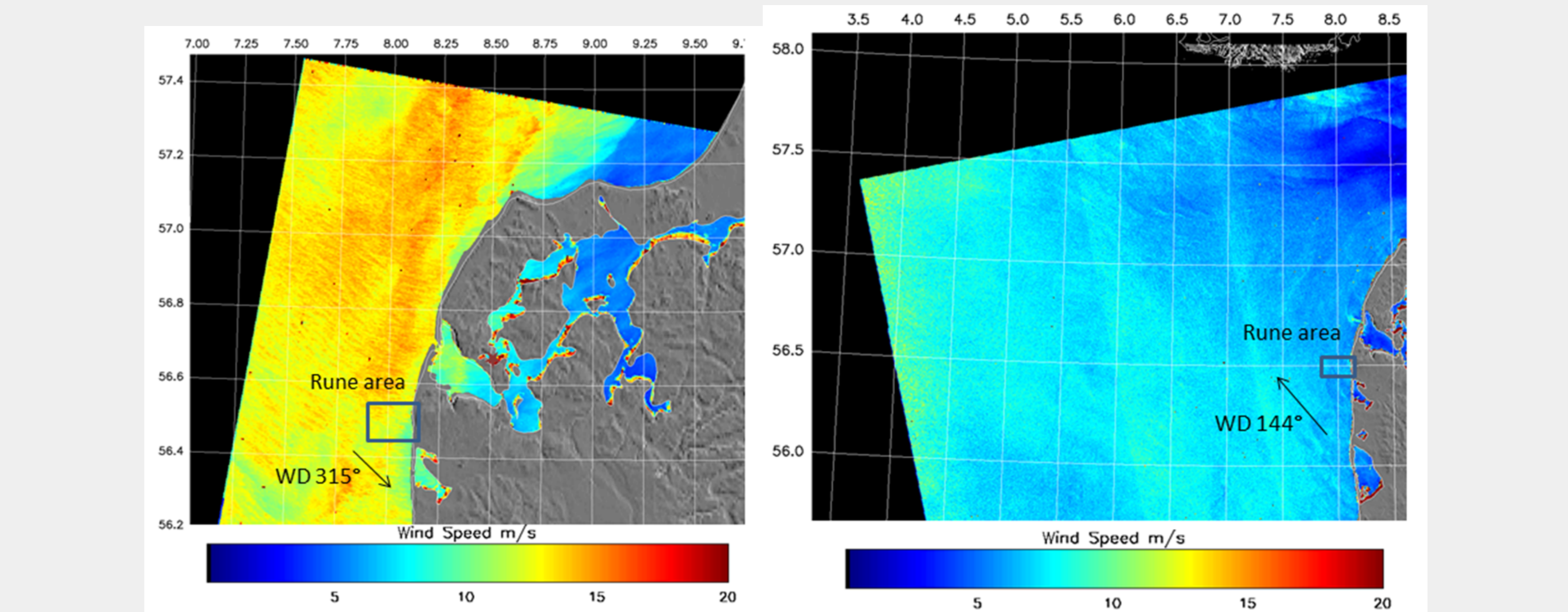
Figure 3: SAR wind fields from Sentinel-1A with constant wind direction.
