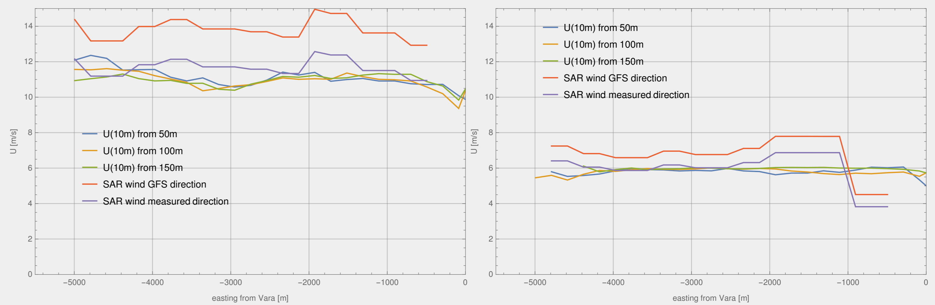
Figure 4: 10m wind speed derived from the three transects and SAR winds retrieval with GFS wind direction input and constant wind direction from dual Doppler measurements.
