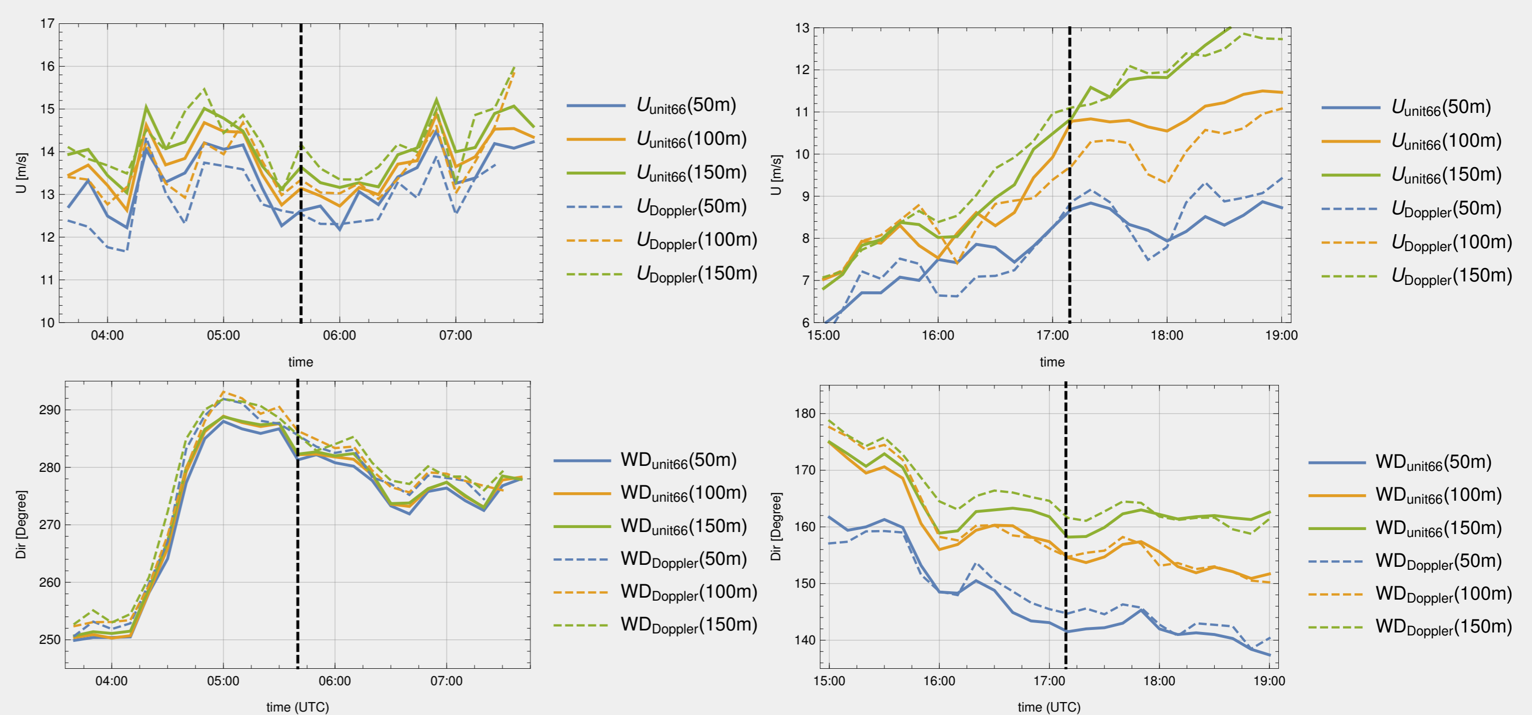
Figure 5: Time series of the wind speed and direction at 50m, 100m and 150m from unit 66 (onshore profiling lidar on the coast at 26.5m height.) and the dual Doppler 1.5km offshore. The black dashed line indicates the time SAR image.
