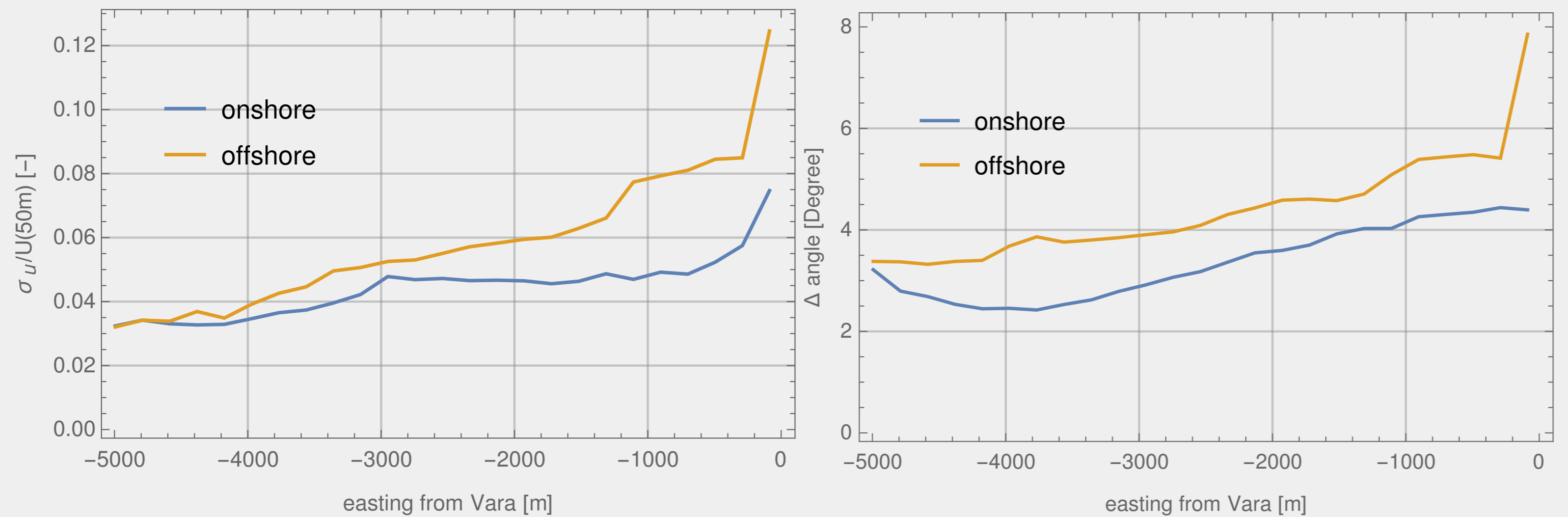
Figure 2: Left: Nondimensional difference between 10m winds derived from 50m and 100m with a logarithmic profile. Right: Difference in wind direction between 50m and 100m. Averaging time from Dec 2015 to Feb. 2016.
