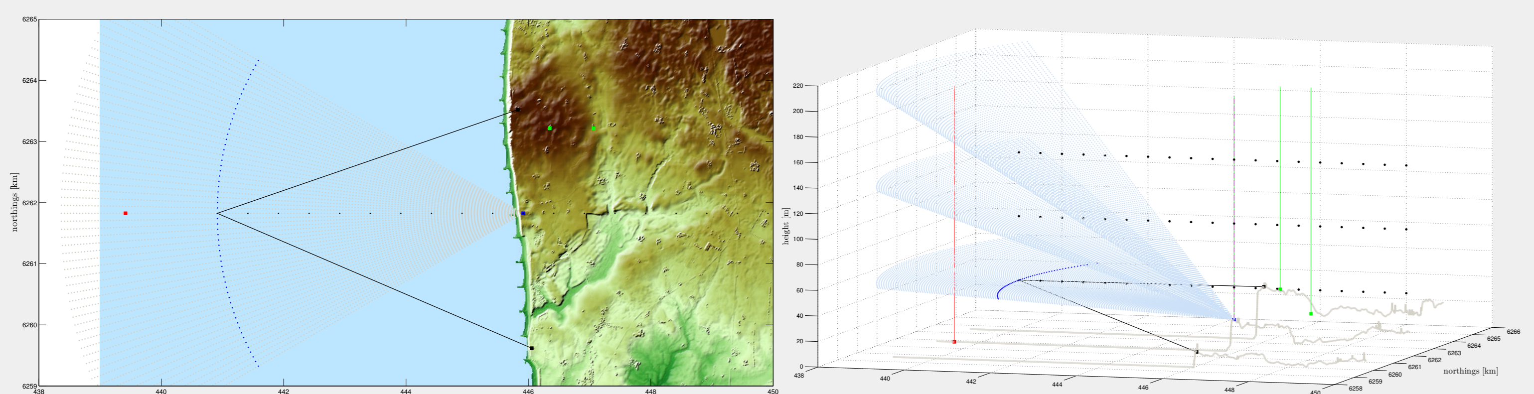
Figure 1: Scanning lidar patterns for RUNE campaign. Sector scans blue, dual Doppler black.
