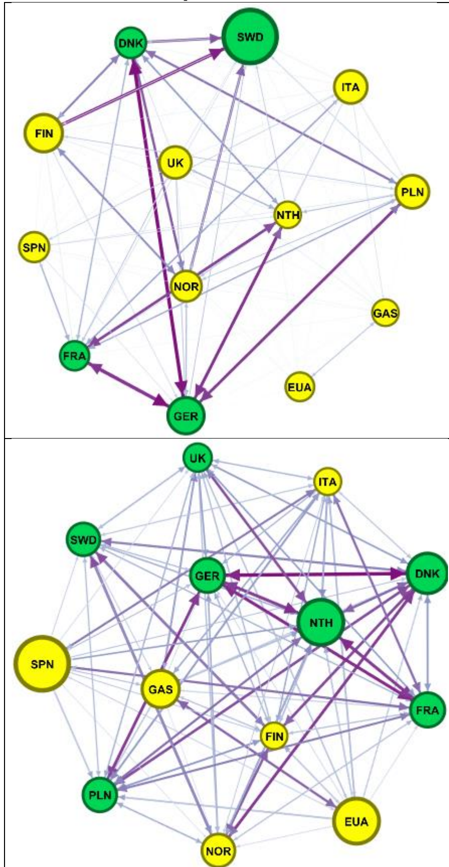
Figure 3. Network connectedness at various quantiles
