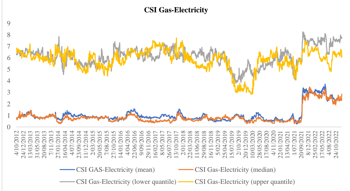
Figure 6. Dynamic CSI_{\text{Gas-Electricity}} at the conditional mean and at various quantiles
